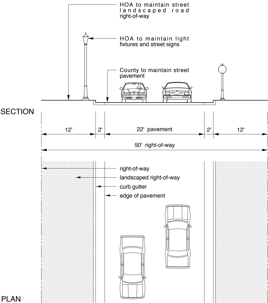
Street Type "A" - Dedicated Street 50' ROW
