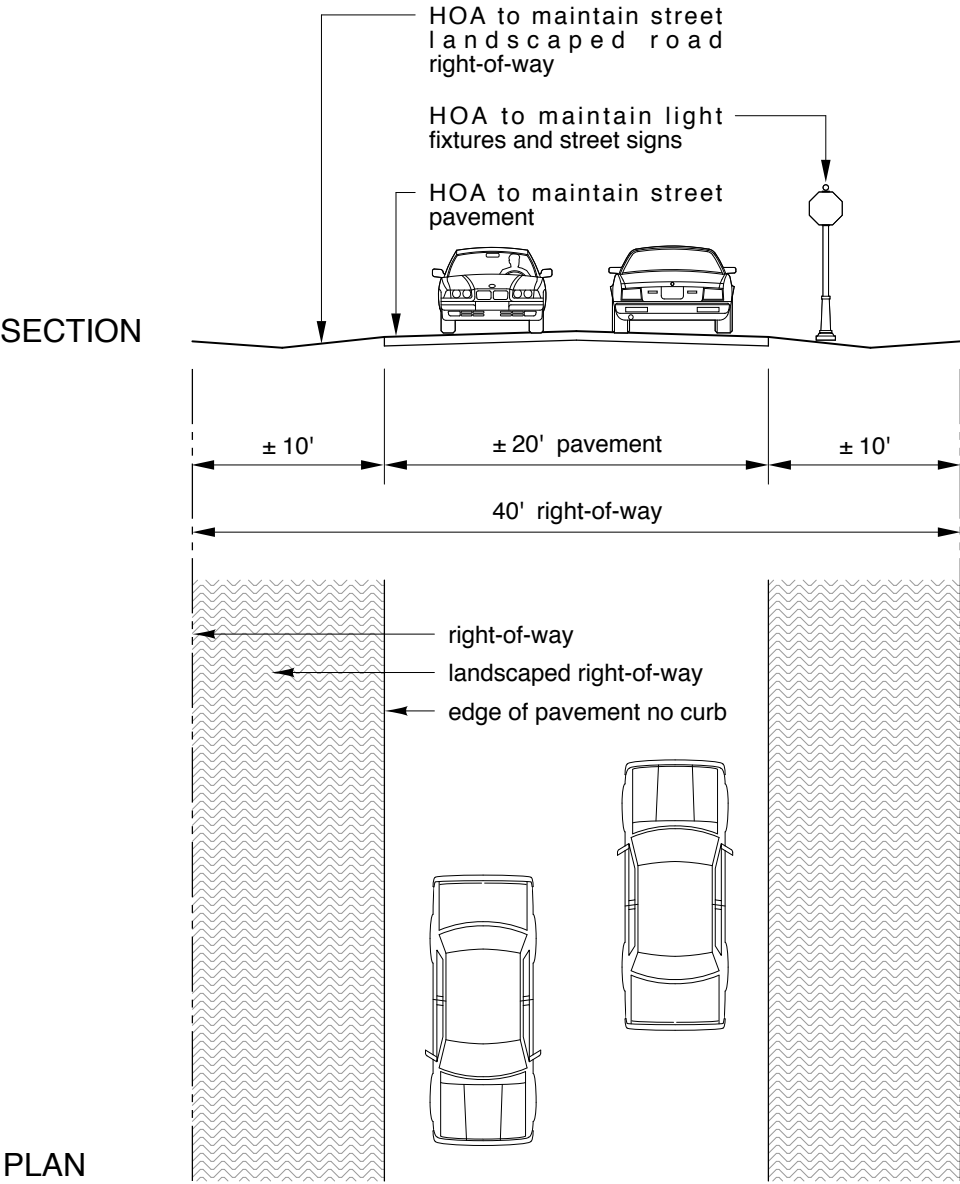
Street Type "C" - Private Street 40' ROW
